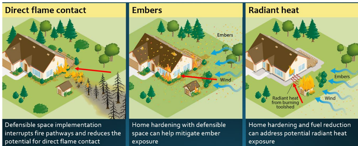
Figure 11: An illustration of the three types of fire exposures that occur during a wildfire. The caption below each panel describes how both defensible space actions, coupled with home hardening measures such as upgraded vents and windows, can help mitigate the exposures and protect buildings from wildfire.
